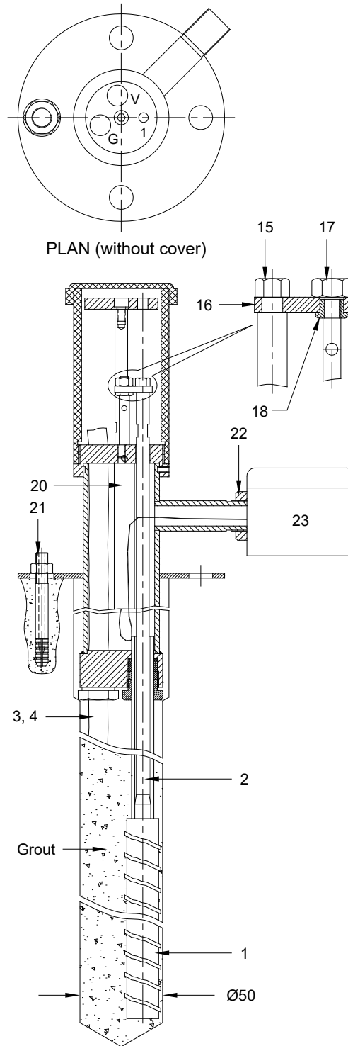
Figure 2.2 - Single point BHE detailed assembly
