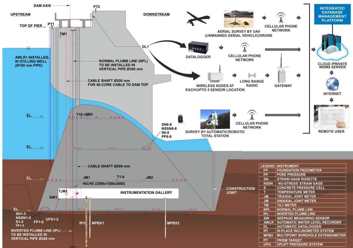
Figure 1: Typical instrumentation scheme of a block of concrete gravity dam
