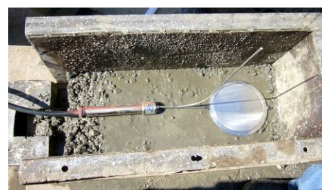
Concrete pressure cell being installed in Ghatgar dam, India
