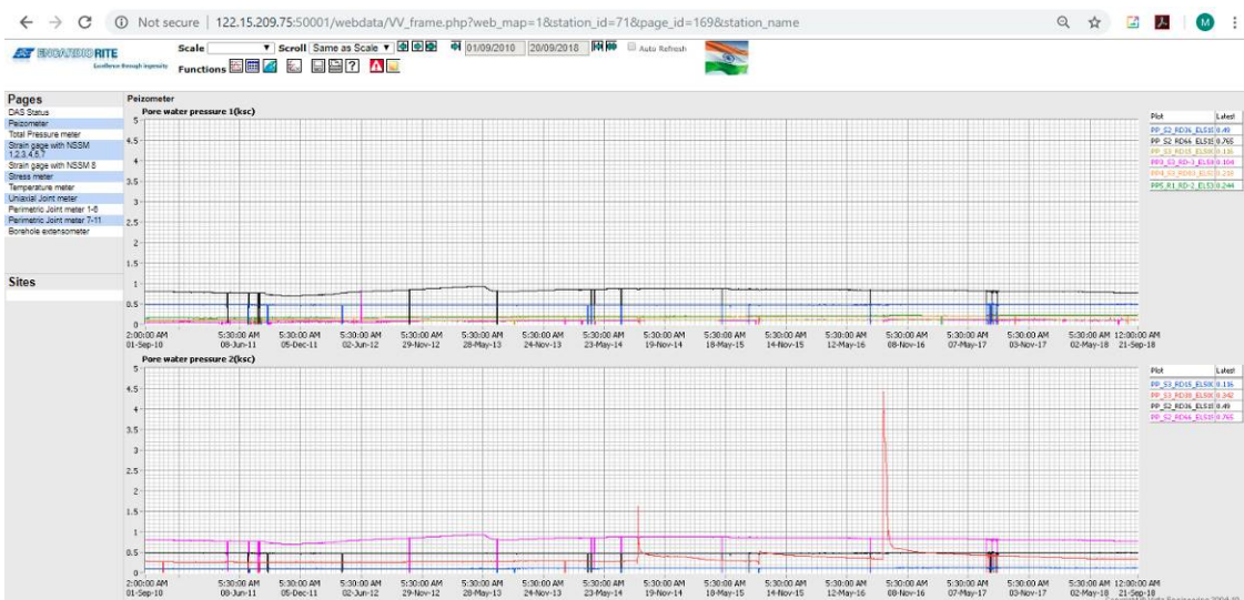
Typical long-term online (8 years) piezometer data from a concrete gravity dam
