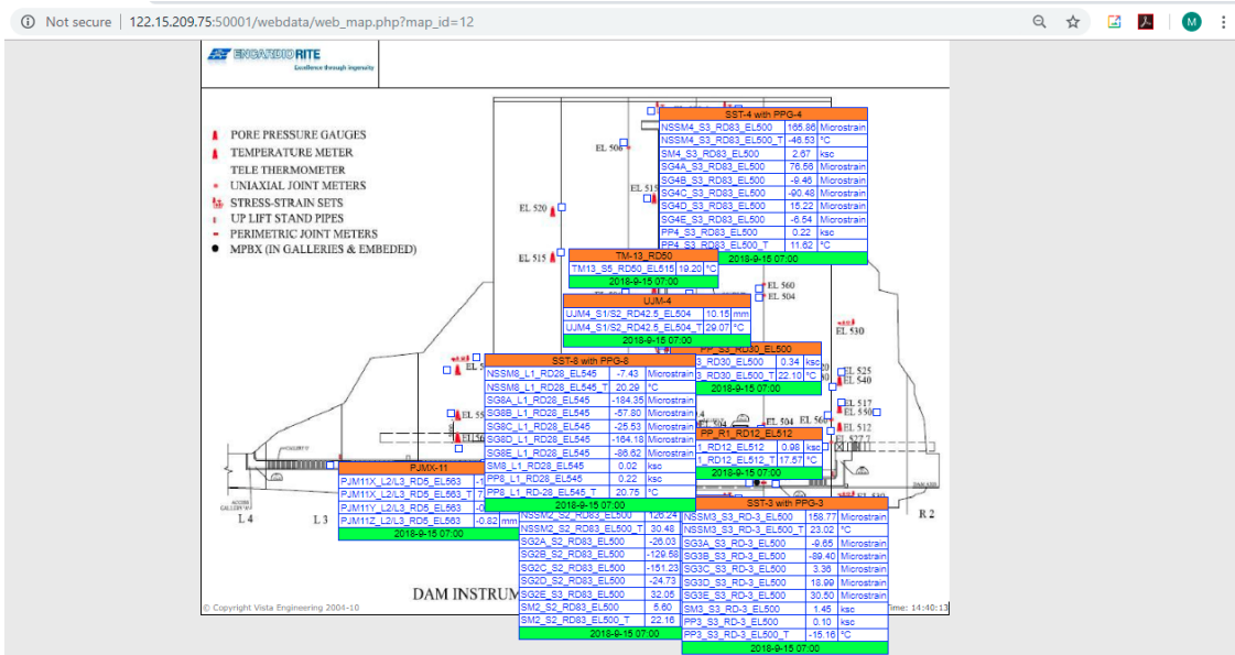
Typical instrument layout scheme with current online data from a concrete gravity dam
